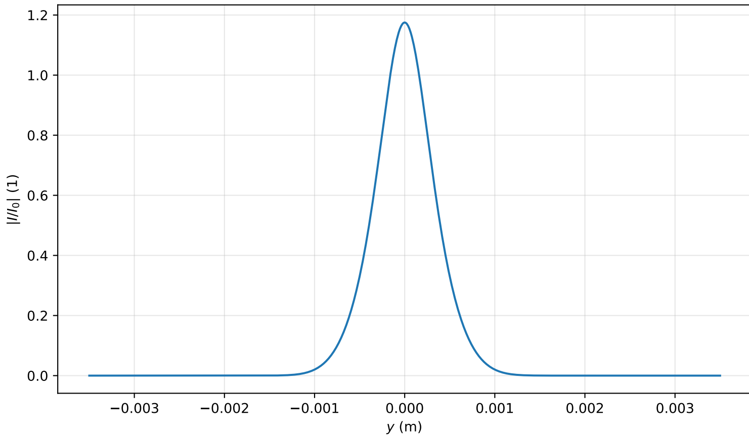
Intensity profile I(x=0, y, z=0.557)/I_0 , P_{in}=0.9P_{cr} , artificial time
